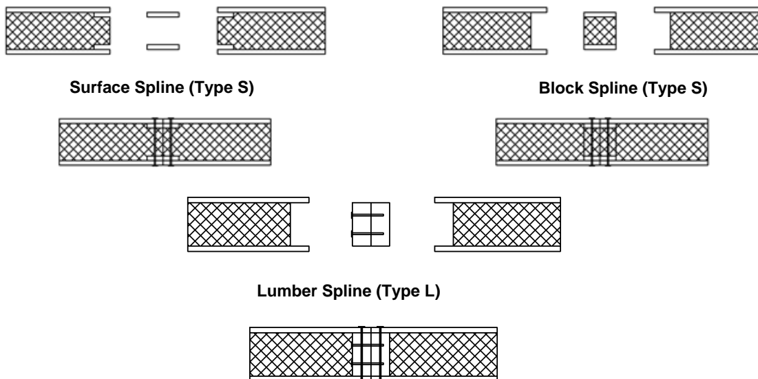
FIGURE 2—SPLINE CONNECTION TYPES
