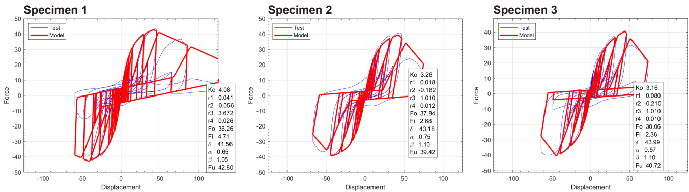
Figure C9. Modified Stewart curves for SIP walls with two 1.2- by 2.4-m panels.
