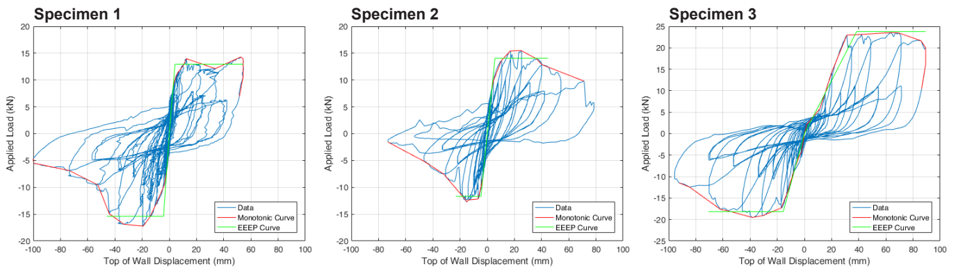
Figure B5. EEEP curves for SIPs with a 1:1 aspect ratio (2.4 by 2.4 m).
