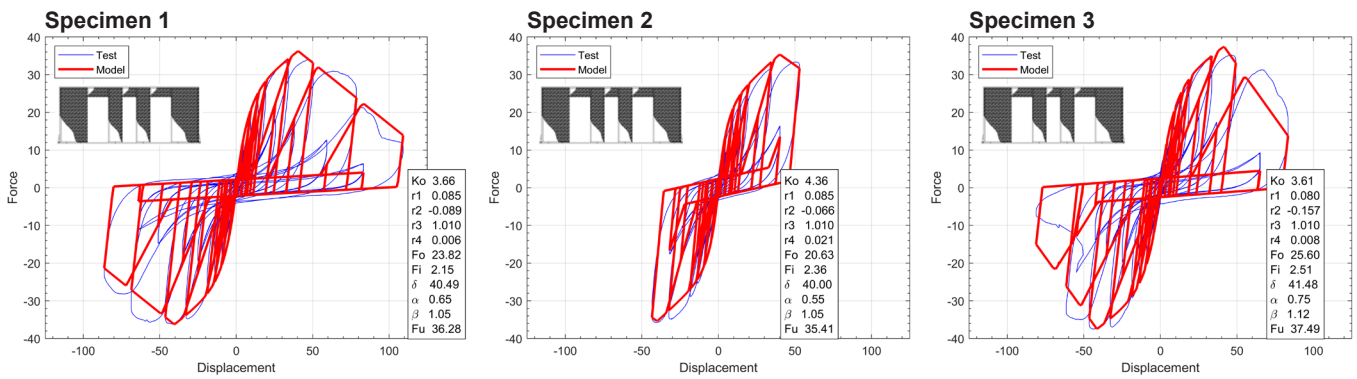
Figure C12. Modified Stewart curves for 6.04-m SIP walls with openings—configuration 201.
