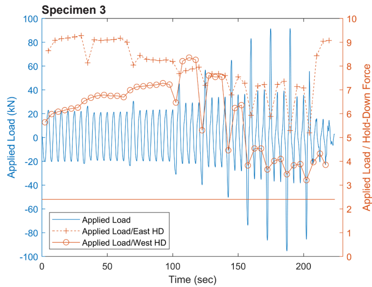
Figure D7. Ratios of applied load to hold-down force for multiple-panel SIPs without openings: five panels.
