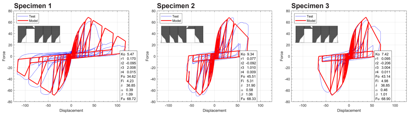
Figure C14. Modified Stewart curves for 6.04-m SIP walls with openings—configuration 203.
