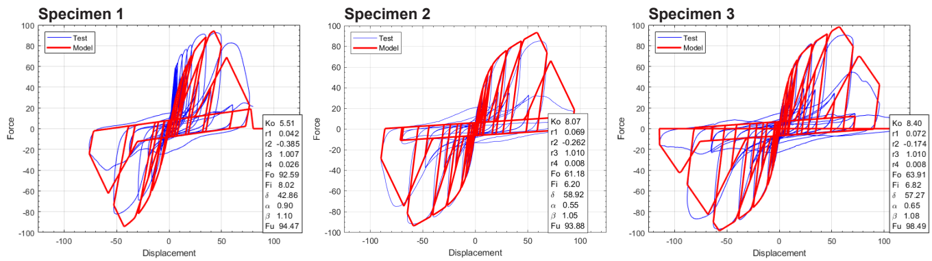
Figure C11. Modified Stewart curves for SIP walls with five 1.2- by 2.4-m panels.
