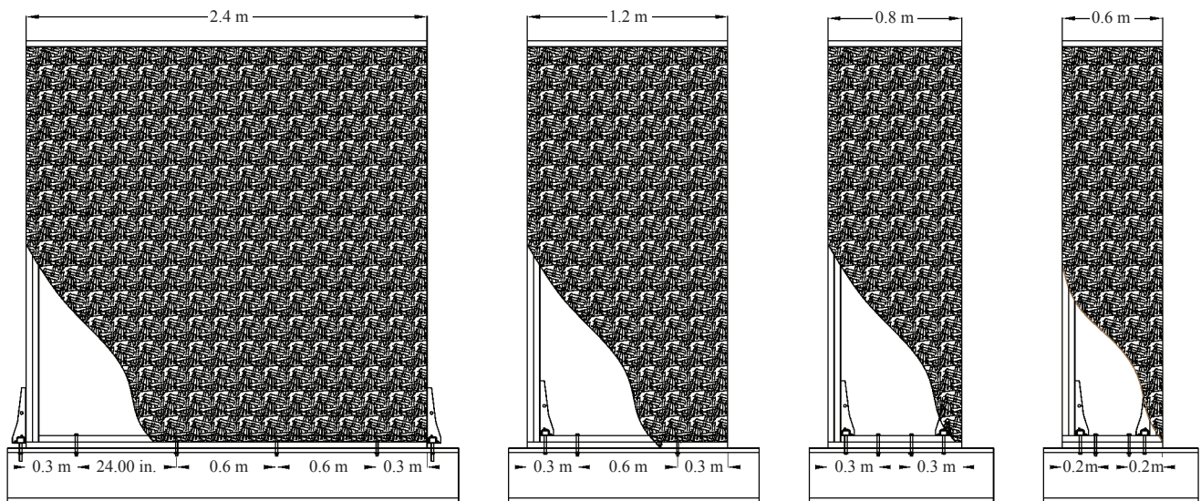
Figure 2. Wall configuration for single-panel SIP wall tests with and without hold-downs.
