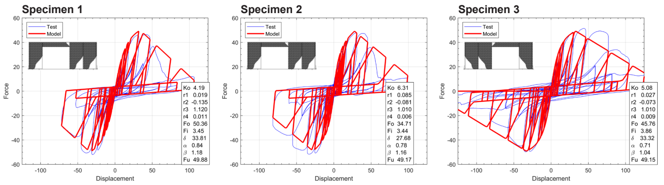
Figure C16. Modified Stewart curves for 6.04-m SIP walls with openings—configuration 205.
