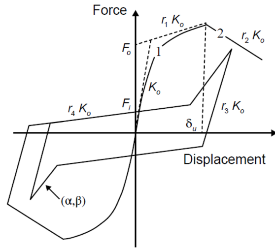
Figure 13. Modified Stewart hysteretic model and associated parameters.
